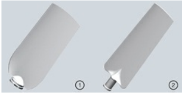
Wide blade design: higher pressure Blade design to ensure the highest efficient airflow performances. Configuration 1: 400 to 630 models. Configuration 2: 710 to 1250 models.
